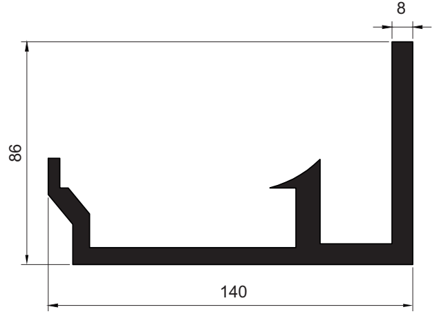
W-103 Wintend Duvar Sabitleme 5,596 kg/m
