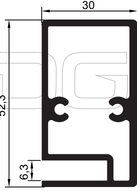
RK-101 Sabit Yatay 1.225 kg/m
