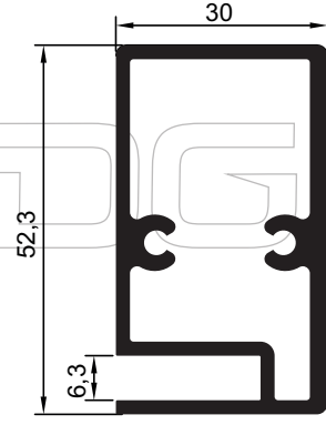
RK-101 Sabit Yatay 1.225 kg/m
