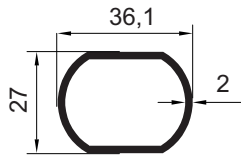
W-104 Wintend Boru 0,542 kg/m
